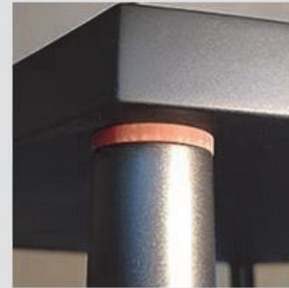
DETAIL 3 DECOUPLING
